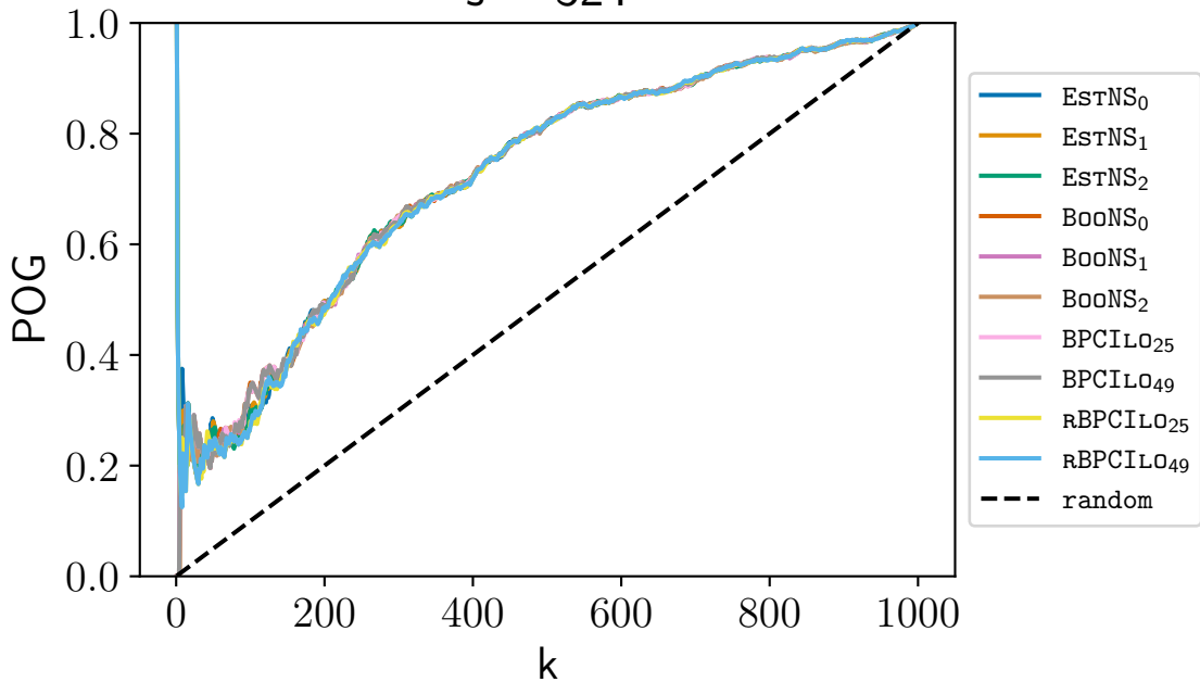
CAT Plot s = 324
